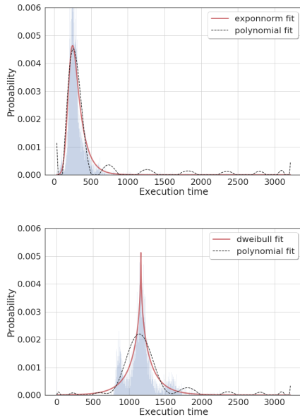
Fig. 1. Performance behavior for two stochastic functions together with two transformations into the continuous domain (top: Functional QA and pre-processing application, bottom: Deep brain structure segmentation application). Runs done during 2017 by the neuroscience department at the Vanderbilt University.
