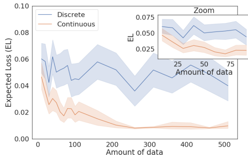
Fig. 5. Results for the sum of truncated normal distributions. For this one we do not plot the semi-clairvoyant algorithm since the cumulative function is not part of the available regular distributions.
