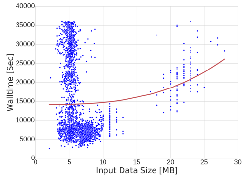
Fig. 2. The relation between the input data size and total execution time for a cortical surface modeling application
