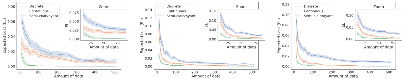
Fig. 4. Results for the truncated normal distributions (left: low variance, middle: high variance) and the truncated exponential distribution (right)
