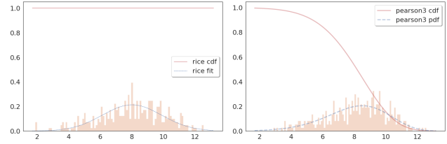
Fig. 9. Behavior of the CDF and PDF for the rice and pearson3 distributions, which best fit the datasets presented.
