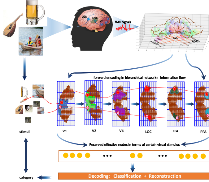
Fig. 1. The framework of our methods.
