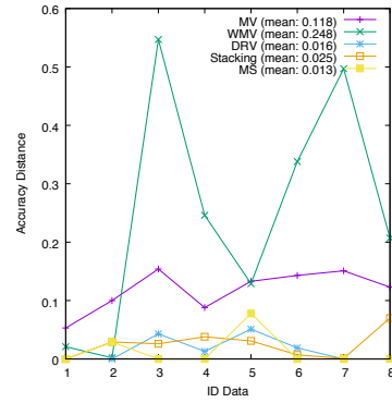
Fig. 3. Accuracy distance before and after 25 spammers were added for eight dataset (smaller value is better).
