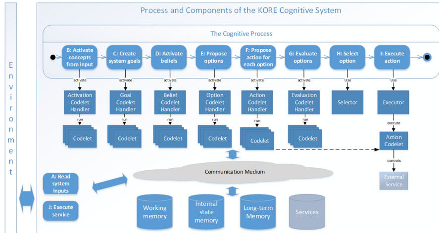
Fig. 4. The cognitive architecture of the project KORE based on the ACONA framework
