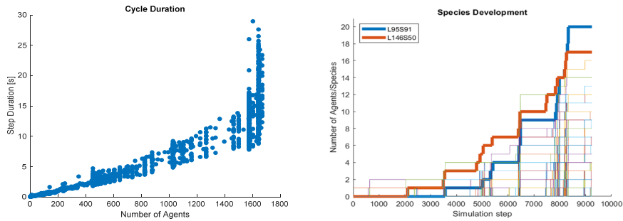
Fig. 6. Left: Cycle duration dependency of the number of trader agents; right: development of species per simulation step
