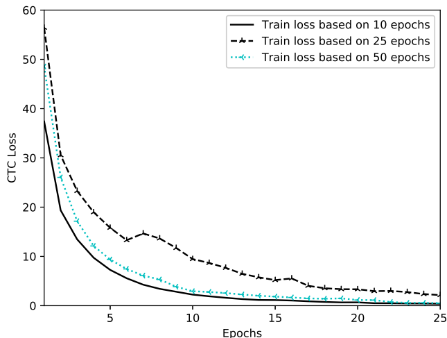
Fig. 10. Random space additional training based on 10, 25 and 50 epochs of synthetic training
