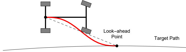
Fig. 3. Quintic spline curve generated by lateral controller, which converges from current state of vehicle to the state of look-ahead point on the path.
