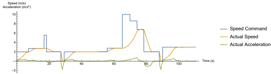
Fig. 11. Experimental results of speed control in simulation.
