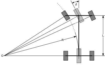
Fig. 2. Ackermann model and bicycle model. Bicycle model simplifies the four wheels of ackermann model into two wheels, centered on the front and rear axles of vehicle.
