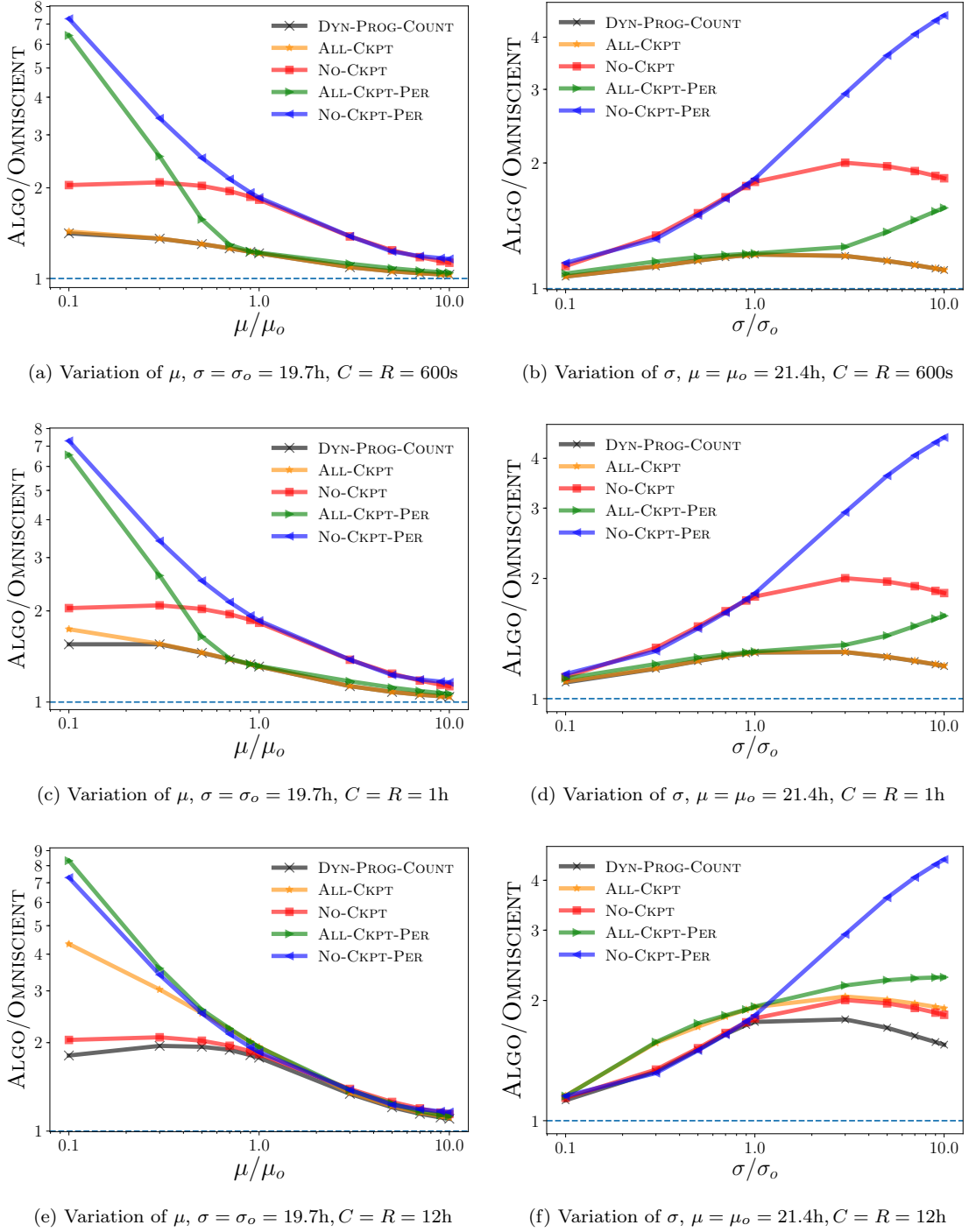
Figure 10: Normalized performance of algorithms with omniscient scheduler when \mu or \sigma vary, using HPC cost function ( \alpha = \beta = 1.0 , \gamma = 0 ). Basis is the Lognormal distribution in Figure 1 ( \mu_o = 21.4h , \sigma_o = 19.7h ). C = R are set to 600, 3600 and 43200s (12h), \varepsilon = 1 .
