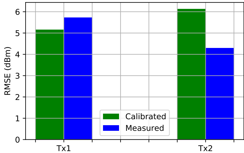
(a) Different transmitted power
