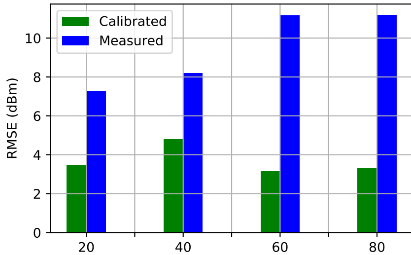
(b) Source position (degrees)
