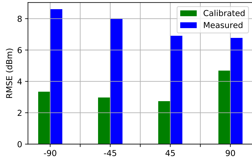
(c) Mainlobe orientations (degrees)
