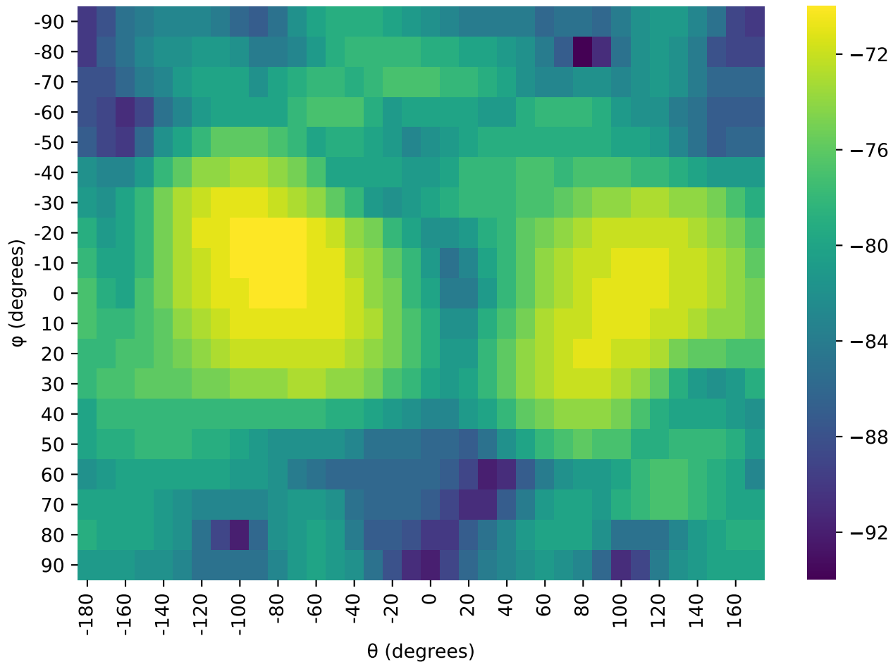
RX heatmap
