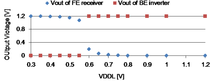
Fig. 8. Output voltages of the FE NAND receiver and the BE inverter at pRBB=2V.
