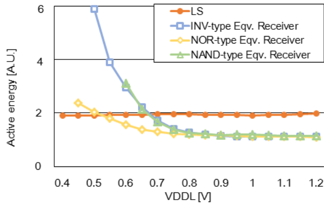
Fig. 15. Active energy of LS and equivalent receivers.
