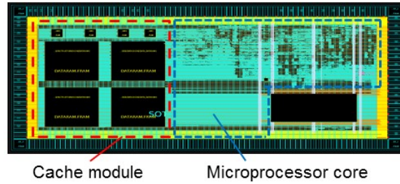
Fig. 19. Layout of the test chip.
