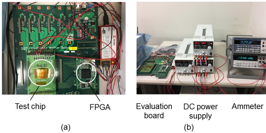
Fig. 20. (a) Evaluation board; (b) Measurement environment.
