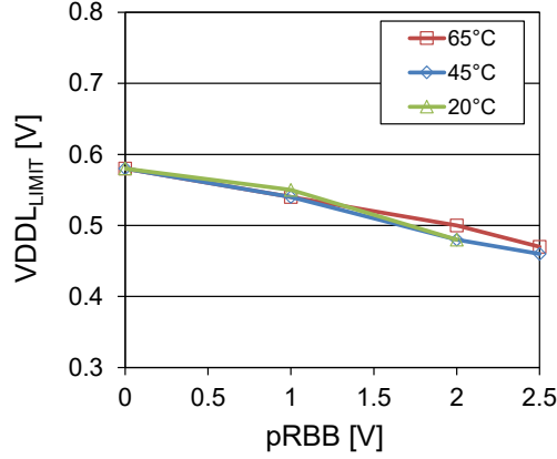
Fig. 21. Measured VDDL LIMIT .
