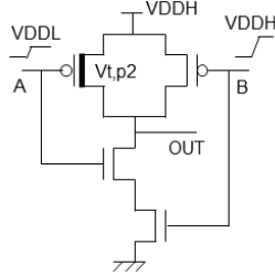
Fig. 3. Level shifting NAND [11].
