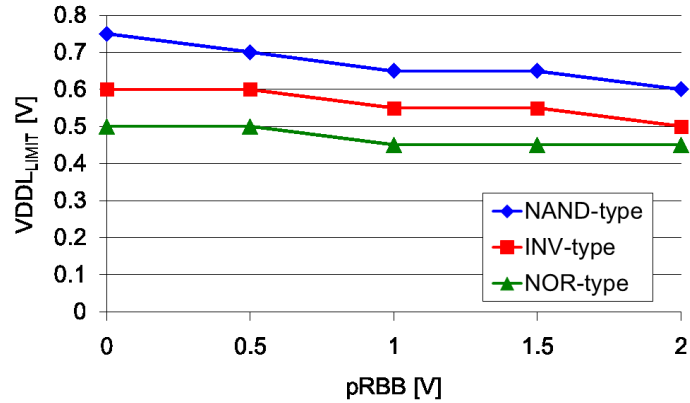
Fig. 9. VDDL_{LIMIT} of equivalent receivers as a function of pRBB voltage.
