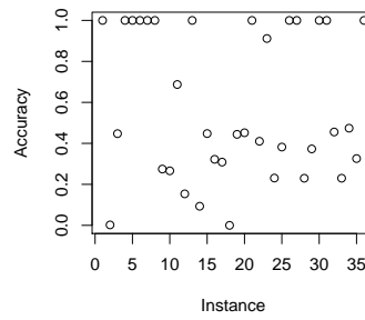
Fig. 29 Testing TNR, 36 clusters, t = 3Q, tolerance H
