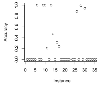
Fig. 27 Testing TNR, 5 clusters, t = 3Q, tolerance H
