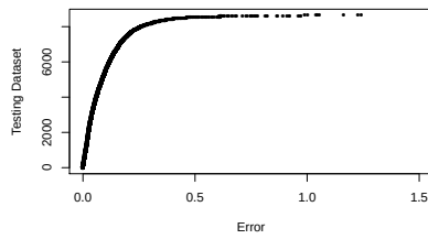
Fig. 19 Testing, CDF of absolute error. \alpha = 1
