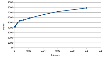
Fig. 5 Average number of positive decompositions (bound)
