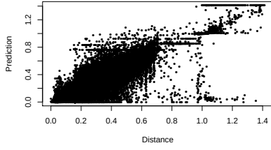
Fig. 16 Training, predicted values over expected ones. \alpha = 1
