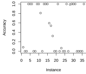
Fig. 26 Testing TNR, 5 clusters, t = median, tolerance H
