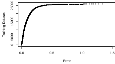
Fig. 18 Training, CDF of absolute error. \alpha = 1
