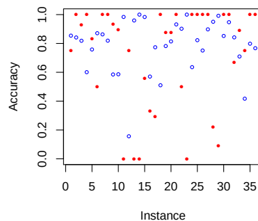
Fig. 23 Testing accuracy
