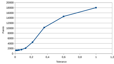
Fig. 4 Average number of positive decompositions (time)
