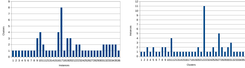
Fig. 25 Clustering with k = 36 , tolerance H. Aggregation by base instance (left) and by cluster (right).
