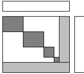
Fig. 1 Structure of a MIP with diagonal blocks (black) and border (grey).
