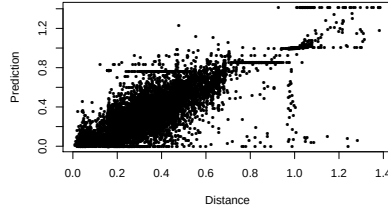
Fig. 17 Testing, predicted values over expected ones. \alpha = 1
