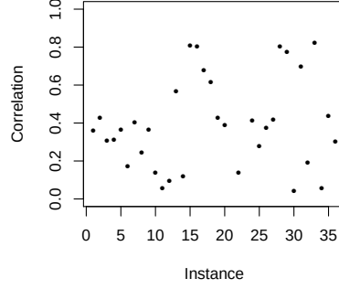
Fig. 12 Third quartile of the distribution of correlation between features and bound.
