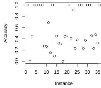
Fig. 29 Testing TNR, 36 clusters, t = 3Q, tolerance H
