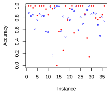
Fig. 22 Training accuracy
