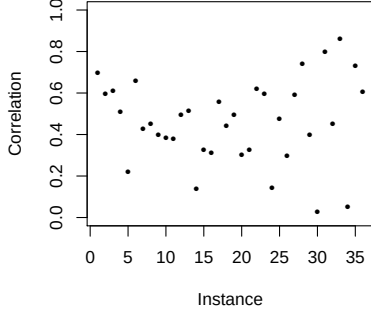
Fig. 11 Third quartile of the distribution of correlation between features and time.
