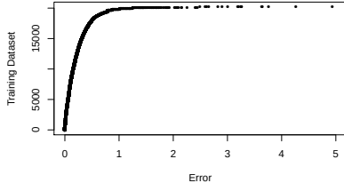
Fig. 20 Training, CDF of MAPE. \alpha = 1
