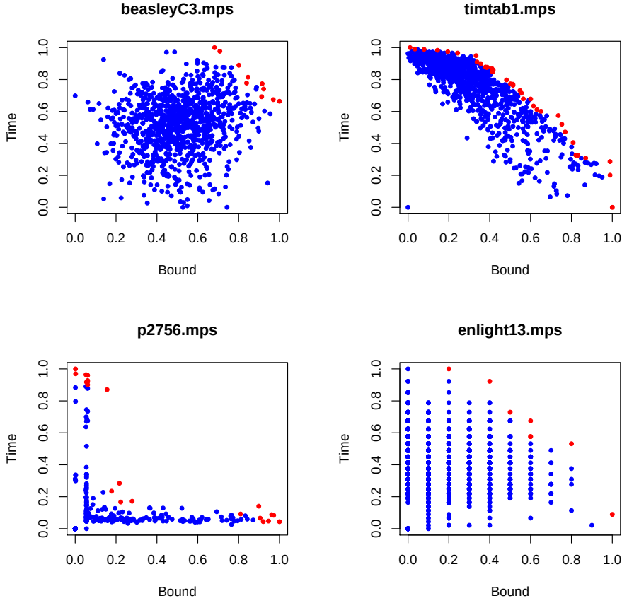
Fig. 6 Bound and time scores for each decomposition on different base instances. Red (resp. blue) points indicate positive (resp. negative) decompositions.
