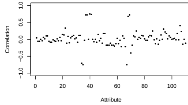
Fig. 15 Correlation between every feature and \delta(\cdot) for \alpha = 10
