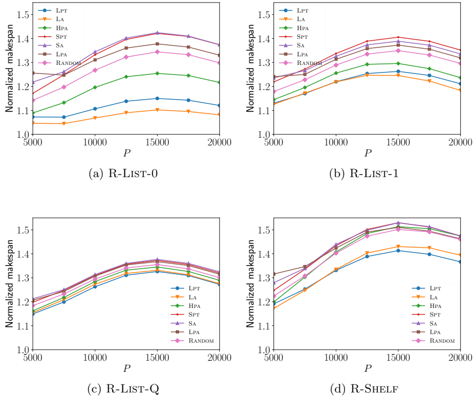
Figure 3: Normalized makespans of different heuristics and priority rules over 30 sets of jobs when P varies between 5000 and 20000, and \bar{q} = 0.3 .
