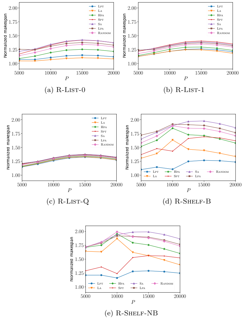
Figure 3: Normalized makespans of different heuristics and priority rules over 30 sets of jobs when P varies between 5000 and 20000, and \bar{q} = 0.3 .
