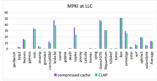
(b) LLC misses per 1000 instructions (MPKI)
