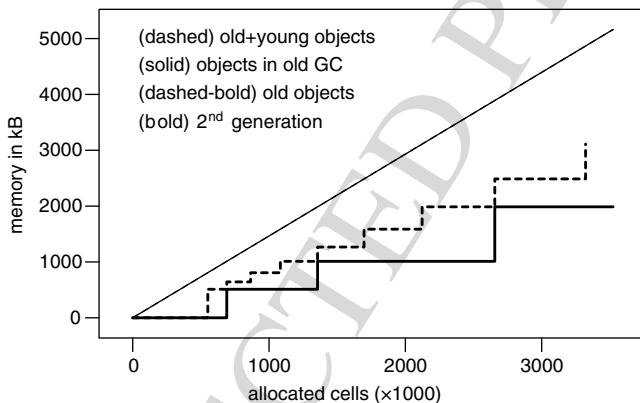
Fig. 5. Memory for 32th Fibonacci number (with sharing).
