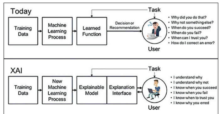
Figure 15: XAI concept
