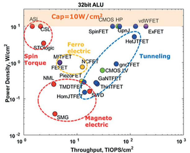
Figure 95: Dissipated power versus computational throughput (capped at 10\text{W}/\text{cm}^2 ) related to a 32-bit ALU Source: [51]
