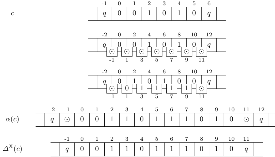
Figure 1. Illustration of a step of the XCA A . The number next to each cell indicates its index in the respective configuration. In this particular example, we use the convention that the \omega\omega -word homomorphism \Phi contracts deleted symbols towards index zero. Adapted from [14].
