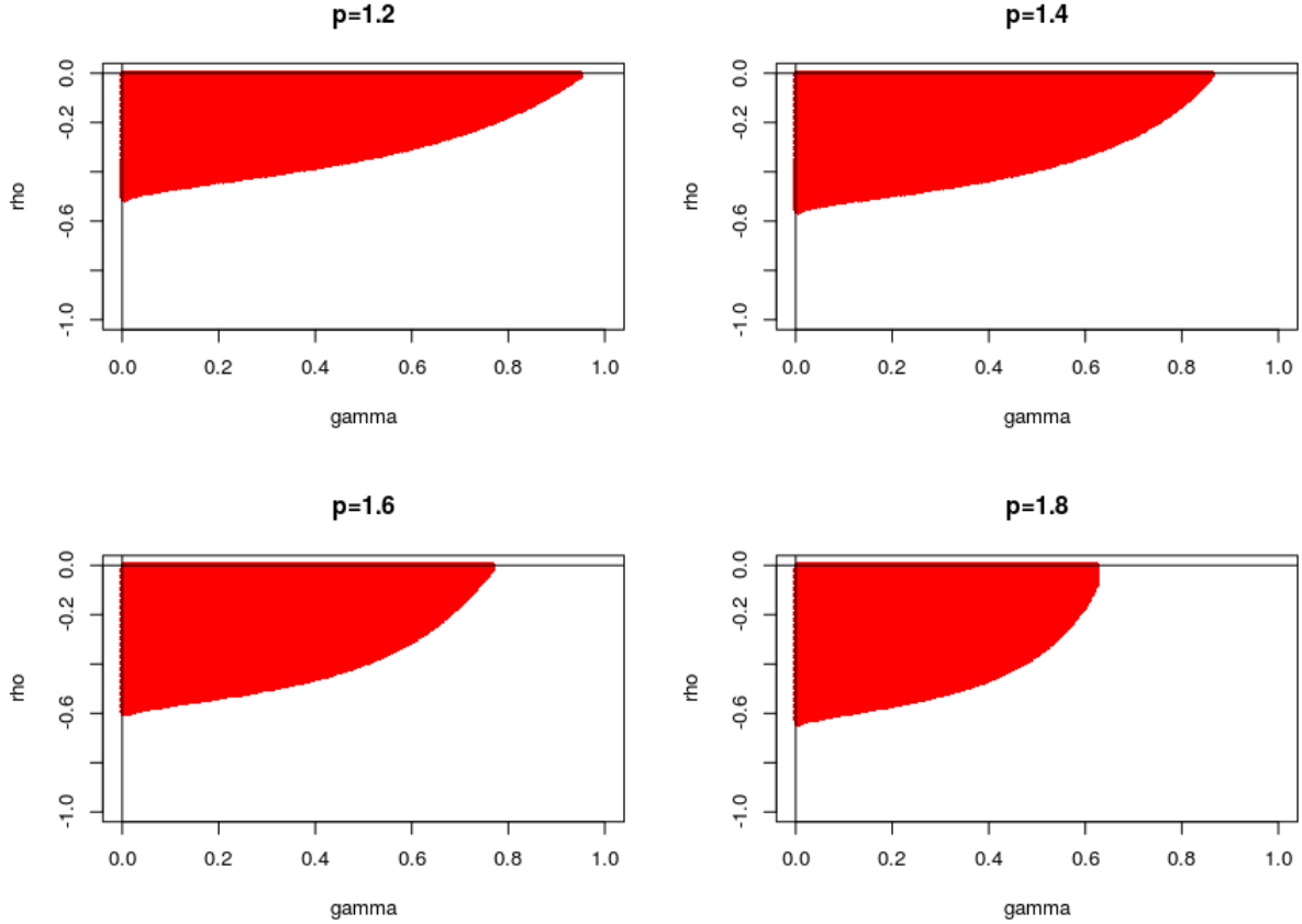
Figure 2: Areas (in red) where the L^p -quantile based tail index estimator has a smaller optimal AMSE than the Hill estimator, for p \in \{1.2, 1.4, 1.6, 1.8\} .
