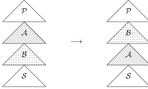
■ Figure 32 vertical- S -swap (special case) from \mathcal{P} \cdot \mathcal{A} \cdot \mathcal{B} \cdot \mathcal{S} to \mathcal{P} \cdot \mathcal{B} \cdot \mathcal{A} \cdot \mathcal{S}
