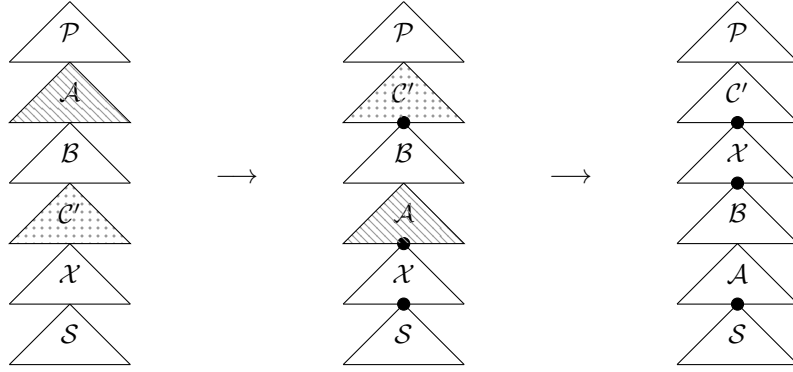
■ Figure 33 The swaps solving the case x_B \prec \varphi(x_A) \prec x_C . The second operation swaps the segments between the dark nodes using Lemma 27.
