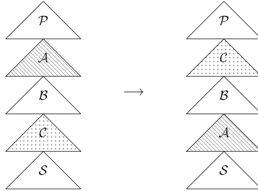
■ Figure 31 A vertical- S -swap from \mathcal{T} to \mathcal{T}'
