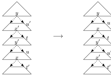
■ Figure 36 We re-associate y to u and x to t with a vertical- S -swap
