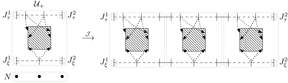
■ Figure 30 Application of \mathcal{J} to \mathcal{U}_+^{[3]} . In this illustration, two jumping pair types \tau and \xi are relevant in \mathcal{U}_+ . The new order <^3 is the concatenation of the old ones
