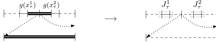
■ Figure 29 From an inclusion g (double line) of the previous \mathcal{V} in \mathcal{R} to the g -border-extension \mathcal{R}_+
