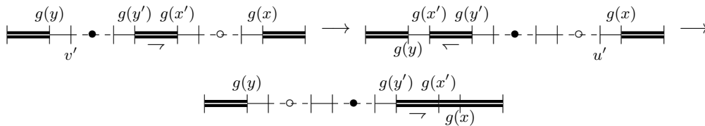
■ Figure 28 Elimination of a jumping pair among two, with two mirror- E -swaps
