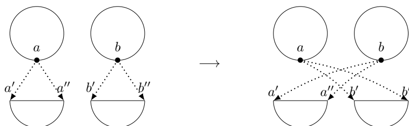
■ Figure 2 The crossing- S -swap between a and b
