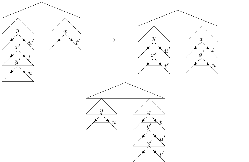
■ Figure 37 We re-associate y to u and x to t with two crossing- S -swaps
