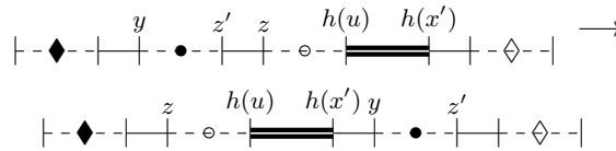
■ Figure 22 An illustration of the progression in the inclusion of \mathcal{V} , if no previous case is applicable
