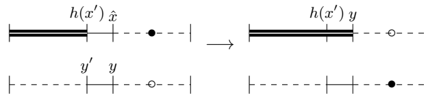
■ Figure 14 An illustration of the progression in the (pseudo-)inclusion (case 1)
