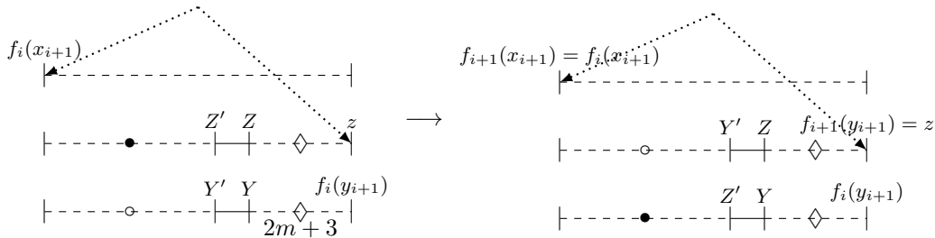
■ Figure 23 After the m -guarded crossing- E -swap between ZZ' and YY' in Q_i , f_{i+1}(x_{i+1}) and f_{i+1}(y_{i+1}) are S -siblings
