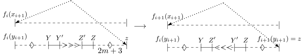
■ Figure 24 After the m -guarded mirror- E -swap at [Z', Y'] in \mathcal{Q}_i , f_{i+1}(x_{i+1}) and f_{i+1}(y_{i+1}) are S -siblings
