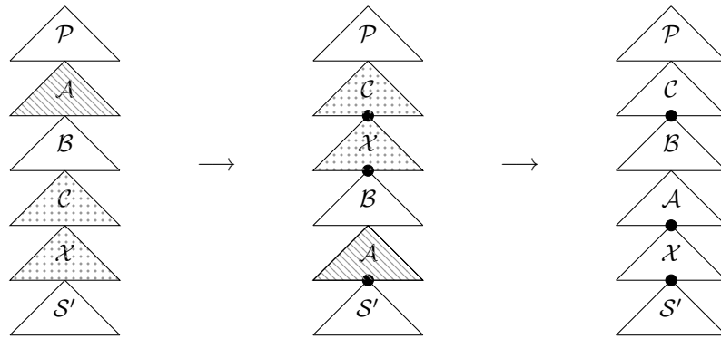
■ Figure 34 The case where x_B \prec x_C \prec \varphi(x_A) . The second operation swaps the segments between the dark nodes using Lemma 27.
