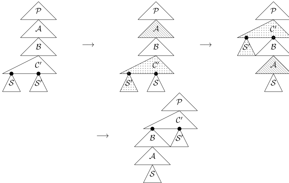
■ Figure 35 The case where x_C and \varphi(x_A) are \prec -unrelated. The first operation is a m -guarded crossing- S -swap between \varphi(x_A) and x_C . The second operation uses Case 1. The last operation is the dual of the first one.
