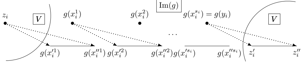
■ Figure 25 From z_i to (z'_i, z''_i)
