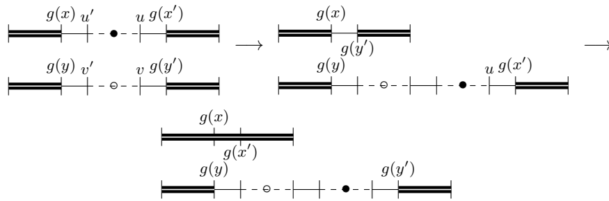
■ Figure 26 Elimination of a jumping pair among two, in different threads
