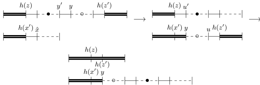
■ Figure 17 An illustration of the progression in the (pseudo-)inclusion (case 4)
