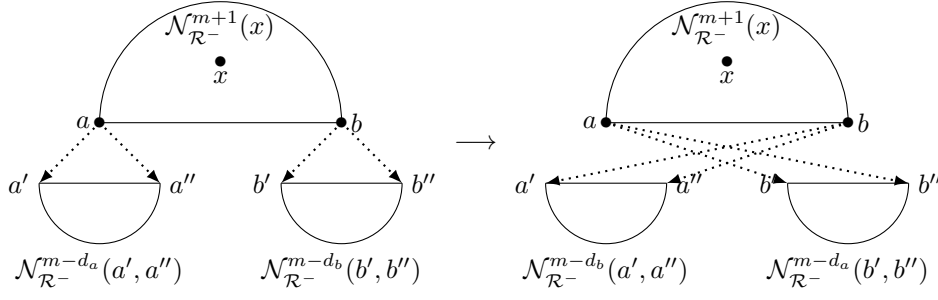
■ Figure 13 Evolution of the neighborhood of x before and after a crossing- S -swap in the proof of Lemma 8. We see \mathcal{N}_{\mathcal{R}^-}^{m+1}(x) on the left and \mathcal{N}_{\mathcal{R}'^-}^{m+1}(x) on the right.
