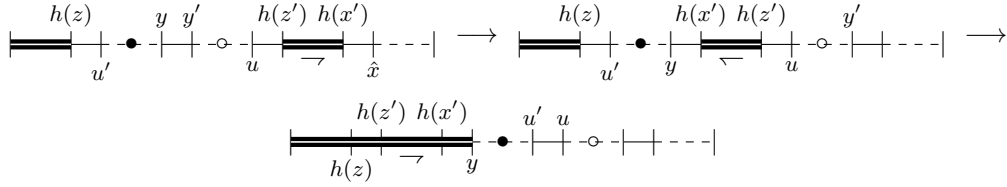
■ Figure 16 An illustration of the progression in the (pseudo-)inclusion (case 3)
