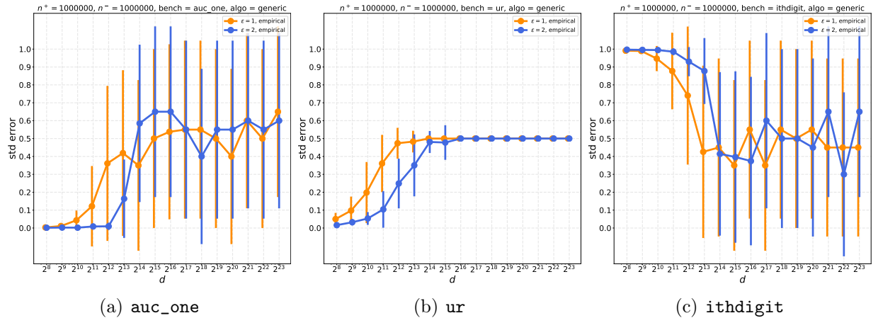
Figure 2: Mean and std. dev. (over 20 runs) of the absolute error of our generic LDP protocol on three synthetic datasets.
