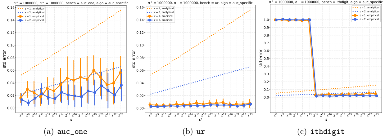
Figure 1: Mean and std. dev. (over 20 runs) of the absolute error of our AUC-specific LDP protocol on three synthetic datasets.
