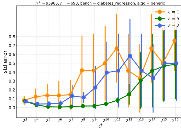
Figure 3: Mean and std. dev. (over 20 runs) of the absolute error of our generic LDP protocol on the scores of a logistic regression model trained on a Diabetes dataset.
