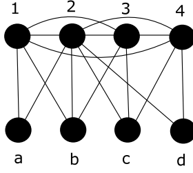
Fig. 1: An interval split graph that is not a clique-interval split graph.
