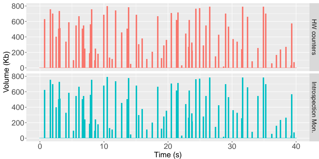
Figure 2: Hardware Counters vs. Introspection Monitoring (time series)
