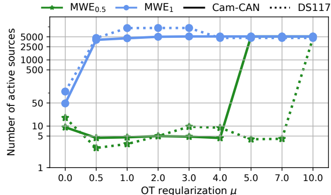
Fig. 5. Number of active sources for MWE models with \lambda = 30\% . The mean is reported across all subjects. With reweighted MWE, a similar phase transition occurs for both datasets after a certain \mu_{\max} .
