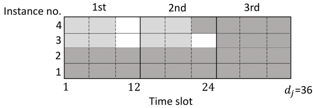
Fig. 3. Illustration of the process of allocating instances to j where a_j = 1 , d_j equals 3 hours, L = 5 minutes, z_j = 132 , and \delta_j = 4 : the light gray (resp. heavy gray) area in every period of [12 \cdot (i - 1) + 1, 12 \cdot i] illustrates the workload processed by spot (resp. on-demand) instances in the i -th execution where i = 1, 2 .
