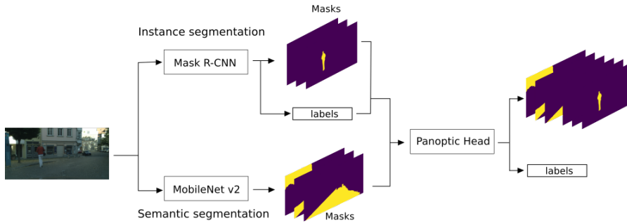
Figure 2: Proposed model
