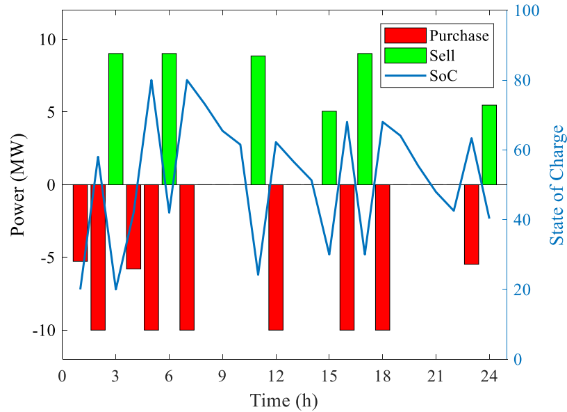
Fig 2. Day-ahead market bids and SoC of the EV fleet.
