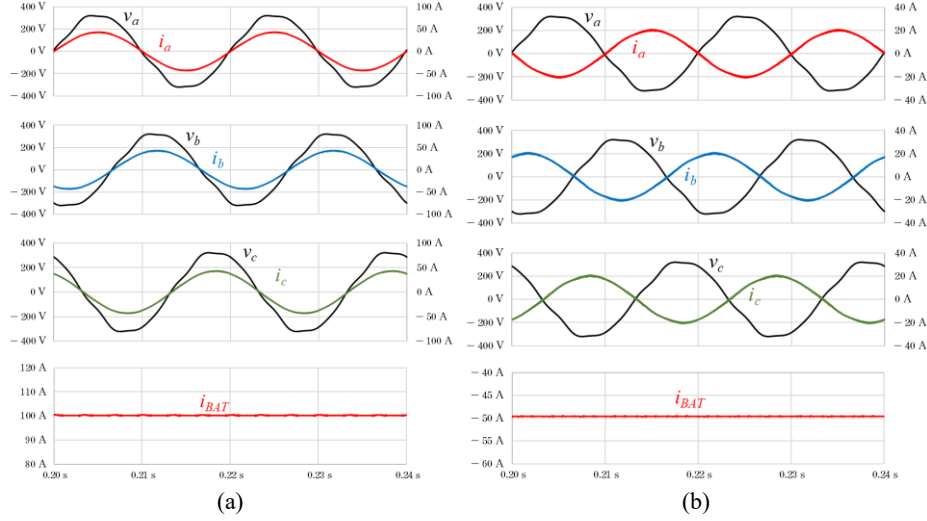
Fig. 5. Simulation results of the proposed system during the interface with a three-phase AC power grid: (a) G2V operation; (b) V2G operation.
