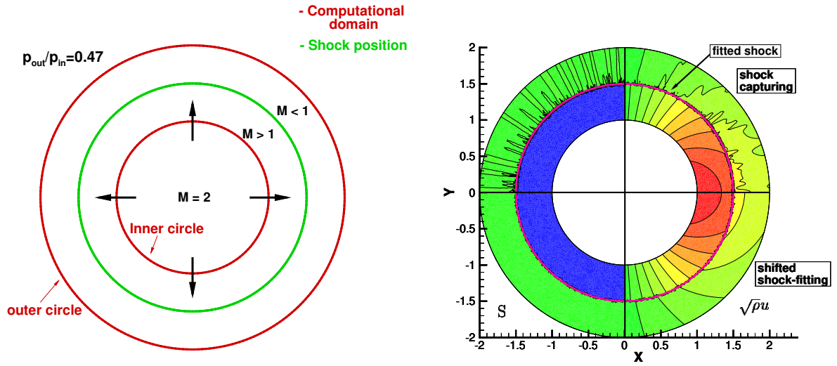
(a) Computational domain and boundary conditions. (b) Entropy, S , in the 2 nd and 3 rd quadrant and \sqrt{\rho}u iso-lines in the 1 st and 4 th quadrant.
