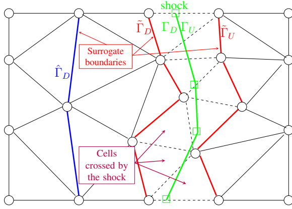
Figure 2: Cell removal across the shock polyline
