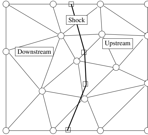
Figure 1: Shock front moving over the CFD mesh
