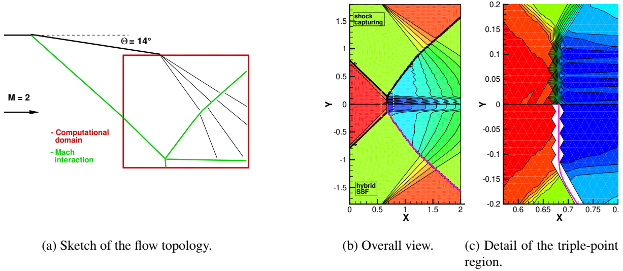
Figure 9: Steady Mach reflection: comparison between the Mach number isocontours computed by means of SC (upper frames) and SSF (lower frames); the fitted shock is shown using a bold solid line.
