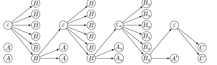
Figure 5. Example of instance built with m = 6 , k = 2 . Note that this instance contains 1 subphase of subtasks denoted by the subscript s .
