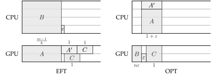
Figure 6. Schedule obtained by EFT (left) and an nearly-optimal one (right). The \varepsilon tasks except the last one are not depicted for simplicity.
