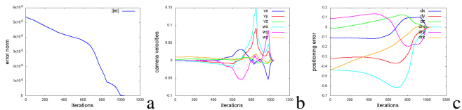
Figure 7. Experiment with Photo-VS and DCT-VS with K = 48400 : (a) \| \mathbf{I}(\mathbf{r}) - \mathbf{I}^* \| or \| \mathbf{f}(\mathbf{r}) - \mathbf{f}^* \| (b) camera velocity (in m/s and rad/s) (c) positioning error (in m and rad).
