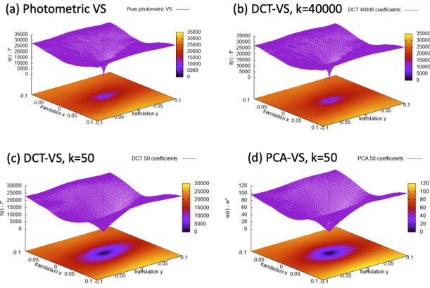
Figure 3. Cost function of various DVS methods (a) pure photometric method [7], (b) DCT-VS with K = 40000 , (c) DCT-VS with K = 50 , (d) PCA-VS [16] with K = 50 .
