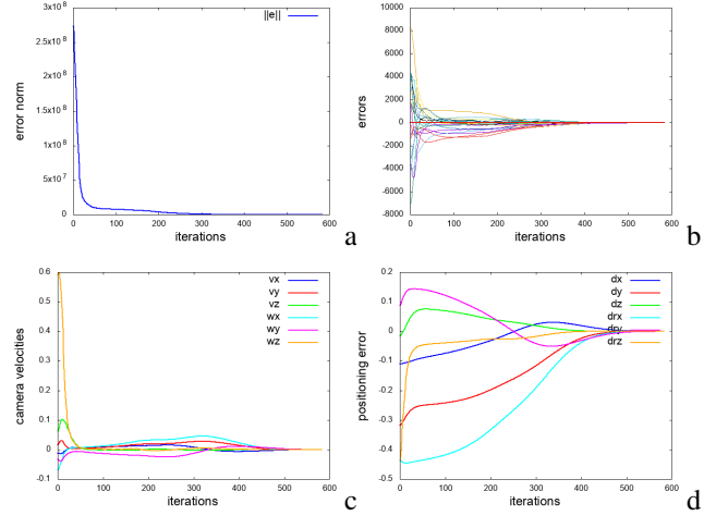
Figure 8. Experiment with DCT-VS with K = 20 (a) \| \mathbf{f}(\mathbf{r}) - \mathbf{f}^* \| , (b) error f_i(\mathbf{r}) - f_i^* , (c) camera velocity (in m/s and rad/s), (d) positioning error (in m and rad).
