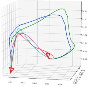
Figure 10. 3D camera trajectories: Photo-VS or DCT-VS with K = 48400 in blue, DCT-VS with K = 10000 in green, DCT-VS with K = 50 in cyan, DCT-VS with K = 20 in red, PCA-VS with K = 50 in purple.
