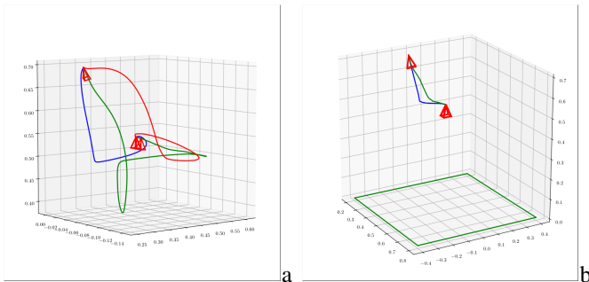
Figure 12. 3D camera trajectories (a) with various number of DCT coefficients (green: K = 10 ; red: K = 20 ; blue: K = 50 ) (b) comparison with PCA-based visual servoing [16] (green: PCA-VS, blue: DCT-VS)
