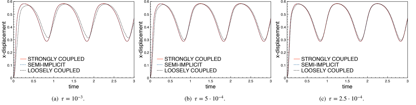
Figure 7 Time evolution of the x-displacement for the structure endpoint B .
