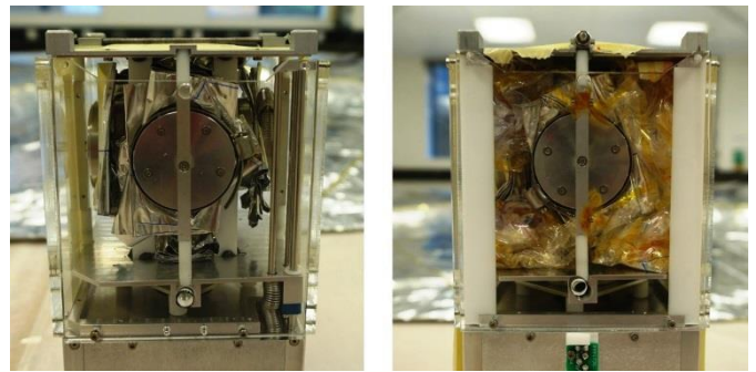
Figure 10: DS-1: Packaged Inflation Module.
