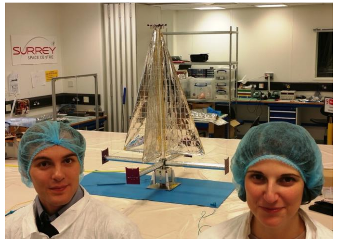
Figure 11: DS-1: FM CubeSat SEET Inflation. This figure shows the DS-1 CubeSat under a final deployment test as part of the SEET.
