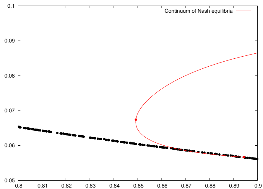
Figure 15: Sandwich panel prioritized optimization - Functions along the continuum
