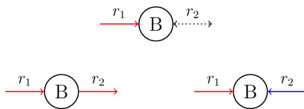
Fig. 1. Reversible reactions can have two different assumptions of a shift that result in the same changes in metabolite balances. The increase in flux in r_1 implies that either more of B should be consumed or less produced in reaction r_2 , depending on its direction. Both of these scenarios correspond to \Delta \mathbf{v}_2 > 0 but the colour given to r_2 , either red for an increase (left) or blue for a decrease in flux (right), depends on the interpretation
