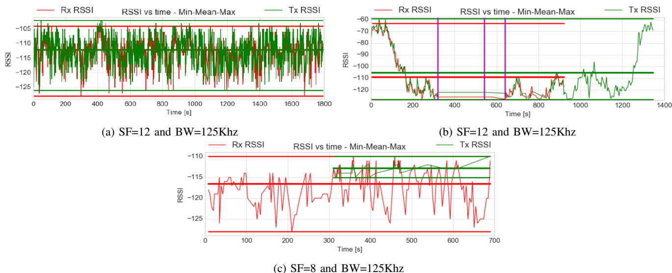
Fig. 2: RSSI value over time
