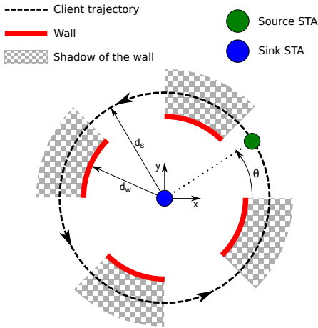
Figure 4: Scenario 2. Top view of the "Circular Alternating Walls" simulation. Walls create shadows leading to sudden changes in the channel between the source and the sink.
