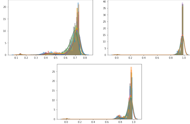
Fig. 6. Distribution of distances in Football obtained using GT (upper left), SimRank (upper right) and ASCOS (bottom). The different colours correspond to the data from different clusters, according to the provided ground truth.
