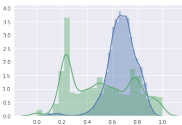
Fig. 8. Distribution of pairwise vertex distances without preprocessing (blue) and after quantile transformation (green).
