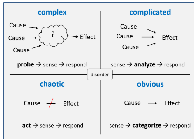
Fig. 2. Cynefin Framework [20]
