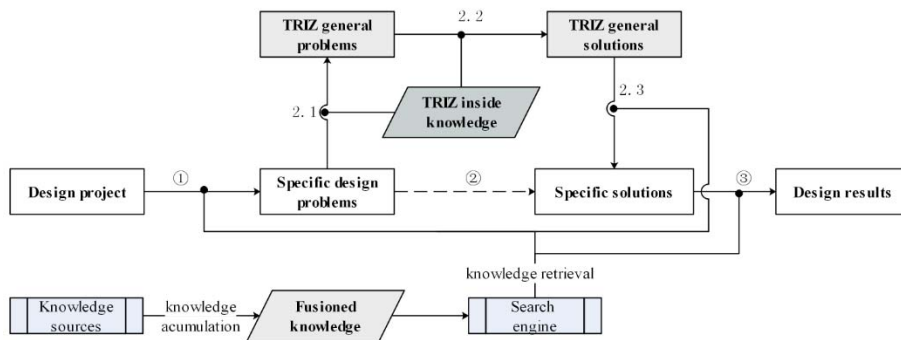
Fig.1. A prototype for a modified TRIZ process integrated with knowledge fusion
