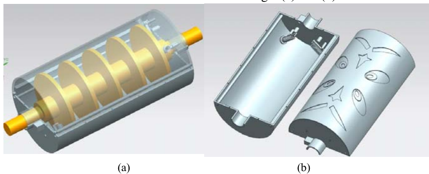
Fig.8. Conceptual solution of the new design solution
