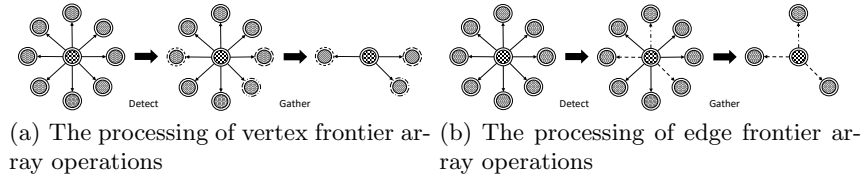
Fig. 4. The processing of frontier array operations: detection and gathering on vertex/edge frontier
