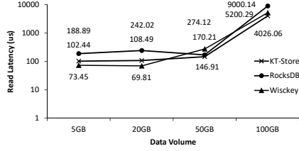
Fig. 10. The average read latencies of KT-Store, RocksDB and Wiskey for the different data volume with the value length of 4KB.
