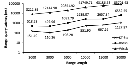
Fig. 8. The average range-query latencies of KT-Store, RocksDB and Wiskey for different range length with the value size as 4KB on HDDs.
