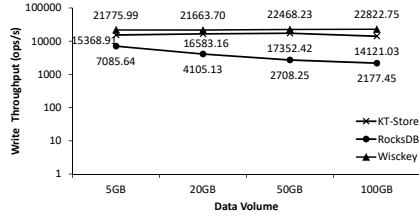
Fig. 7. The average write throughput of KT-Store, RocksDB and Wiskey for the data volumes vary from 5GB to 100GB for a 4KB value size on HDDs.
