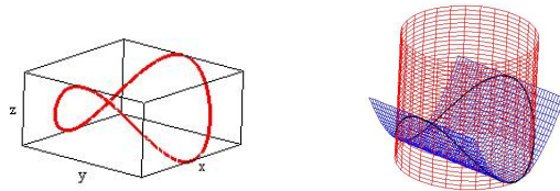
Figure 1: Left: The space curve of Example 3. Right: The two implicit surfaces defining the curve.
