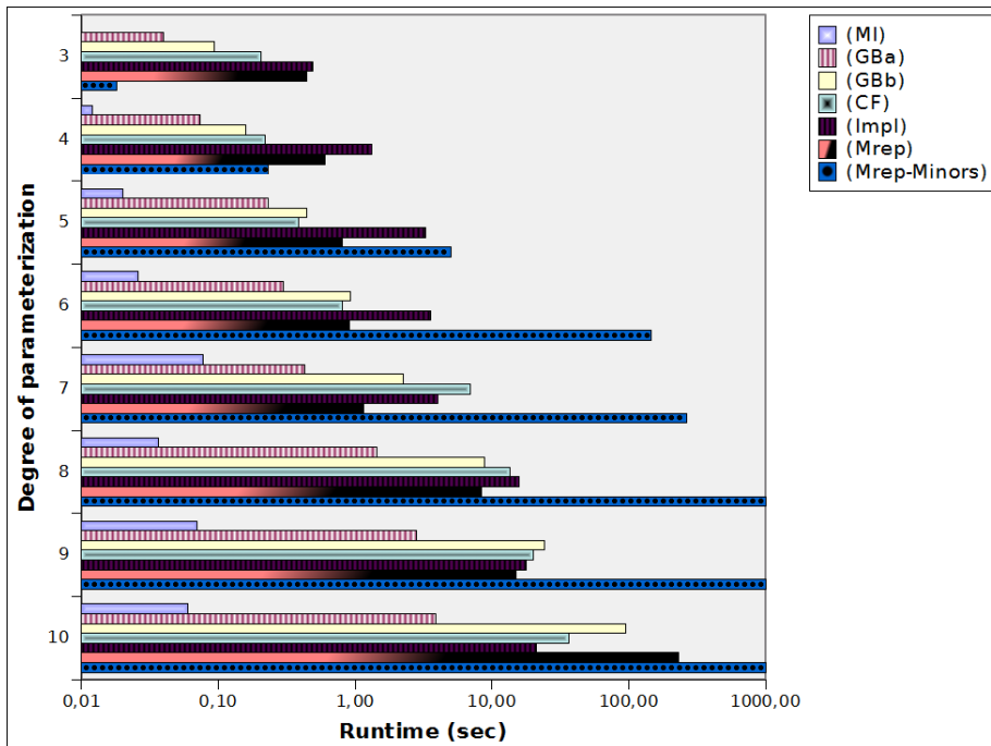
Figure 2: Timing (sec) of various algorithms on random space curves: (CF) implements Alg. 2, (MI) matrix interpolation Alg. 1, (GBa) Gröbner bases by Maple’s Basis , (GBb) Gröbner bases by Maple’s EliminationIdeal , (Mrep) Maple code for matrix representation algorithm using syzygies, (Impl) Maple’s implicitize implementing [4]. (Mrep-Minors) is the time of computing Mrep minors, providing implicit equations. Computing minors by (MI) takes > 20 min at degree 5 thus there is no row for (MI-Minors).
