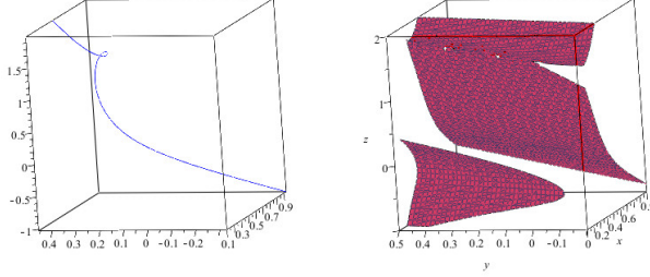
Figure 3: The figures depict the branch of the curve from Example 4 between the two poles (Left) and one of the surfaces computed by the algorithm (Right). The bottom-left component of the surface is "beyond" one of the poles and is disconnected from the other component.
