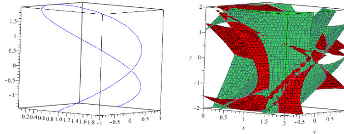
Figure 4: (Left) The curve of Example 9(c.) for a = 1 . (Right) Two of its three defining equations found by Algorithm 2. A third equation is needed in order to remove the extraneous surface intersections.
