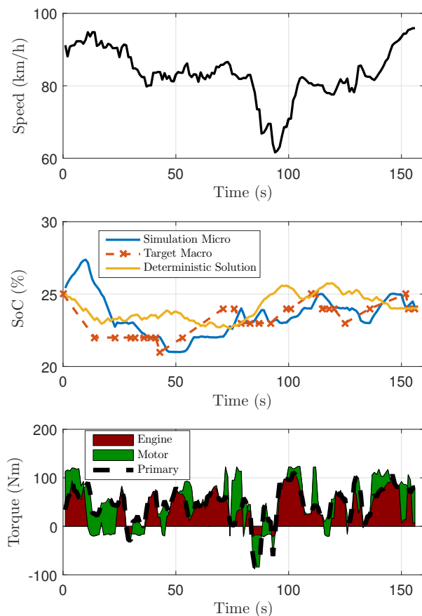
Fig. 12: Macro problem: optimal policy. Bi-level optimization vs DDP. Conditions SoC_0 = 0.25 , SoC_f = 0.24 .
