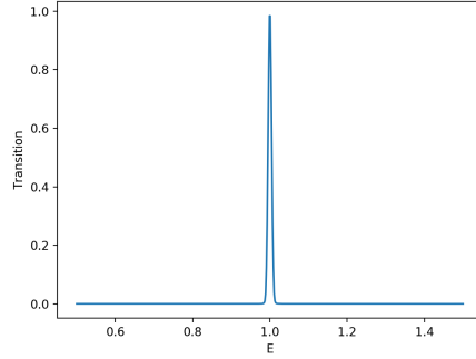
Figure 4: Fidelity |\langle \psi_\epsilon(E, 1), e_2 \rangle|^2 as a function of the drift term E , with \epsilon = 0.01 and \alpha = 1.5 .
