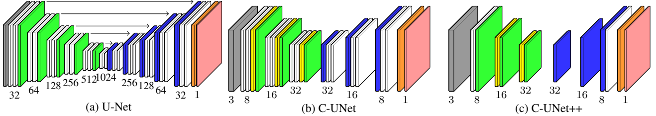
Figure 1: U-Net [31] compared to C-UNet and C-UNet++. Gray: input, white: conv3x3 + ReLU, yellow: depthwise separable conv3x3 + ReLU, green: 2x2 max pool, orange: conv1x1 sigmoid, blue: 2x2 deconvolution, red: output, arrows: skip connections. Numbers indicate the number of feature maps at each stage.
