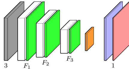
Figure 2: C-FCN and C-FCN++ architectures. Gray: input, white: conv3x3 ReLU, green: 2x2 max pool, orange: conv1x1 sigmoid, blue: 4x4 bilinear upscaling.
