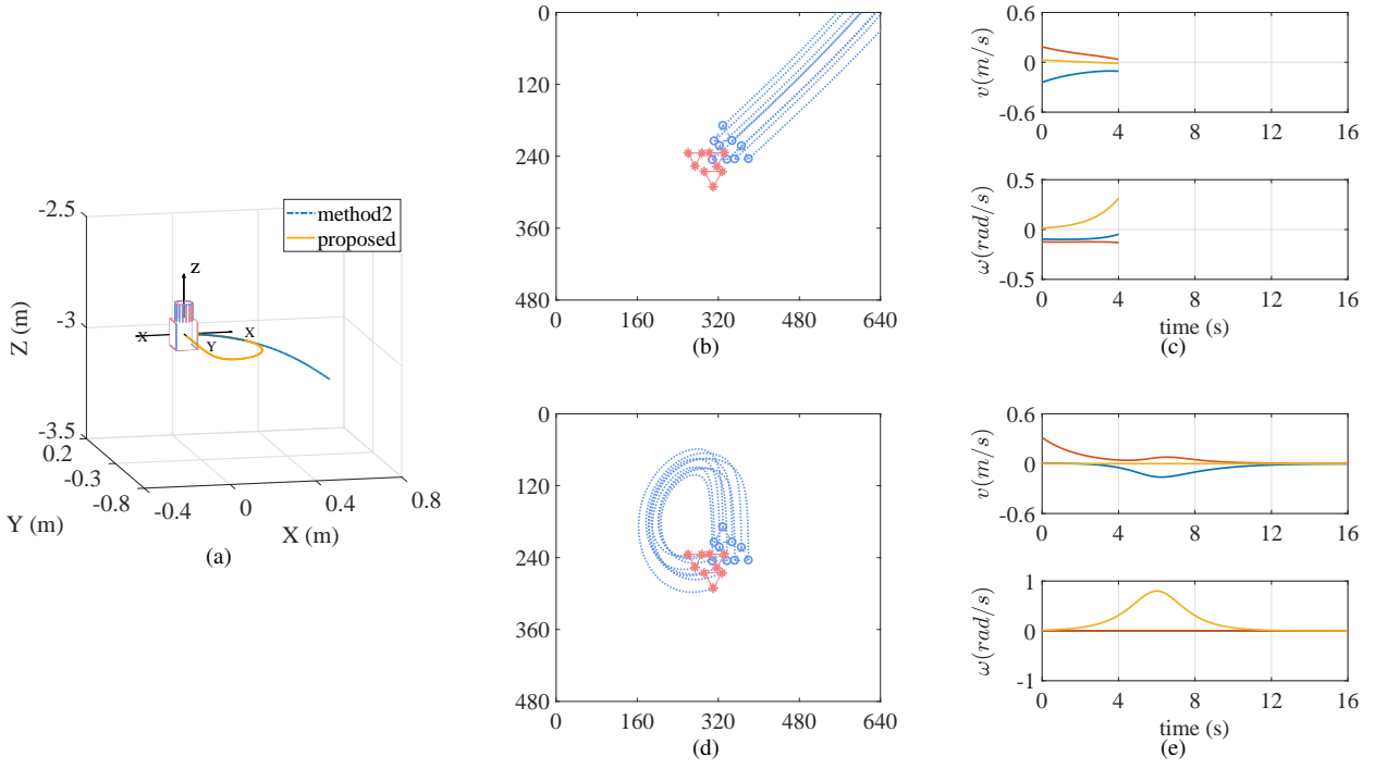
Figure 13. Simulation results with initial system errors close to the equilibrium \Omega_2 and {}^d\bar{t}_i = 0_3 : (a) Camera motion in Cartesian space. (b) Image trajectory of the feature points for method 2. (c) Control inputs for method 2. (d) Image trajectory of the feature points for proposed approach. (e) Control inputs for proposed approach.
