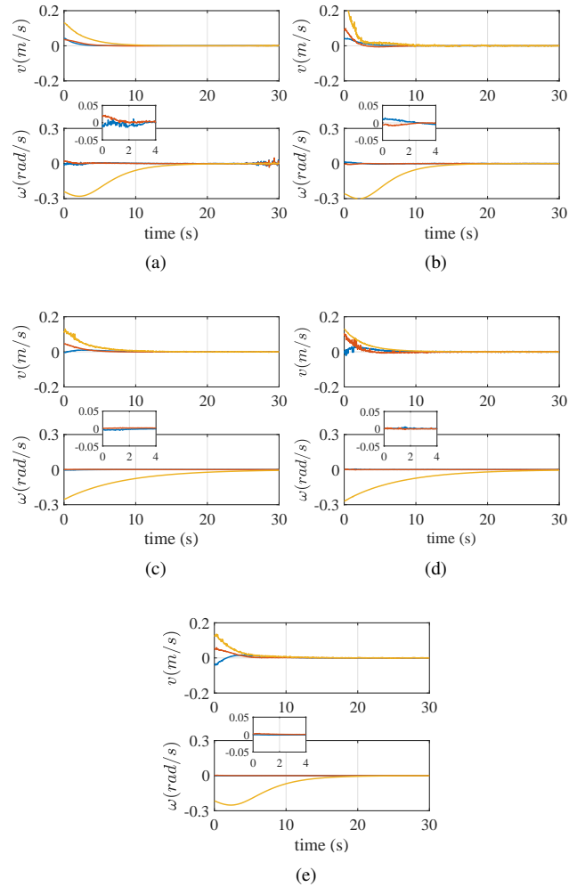
Figure 8. Experimental comparisons of the control inputs for: (a) method 1, (b) method 2, (c) method 3, (d) method 4, (e) and proposed approach in the large rotation case.
