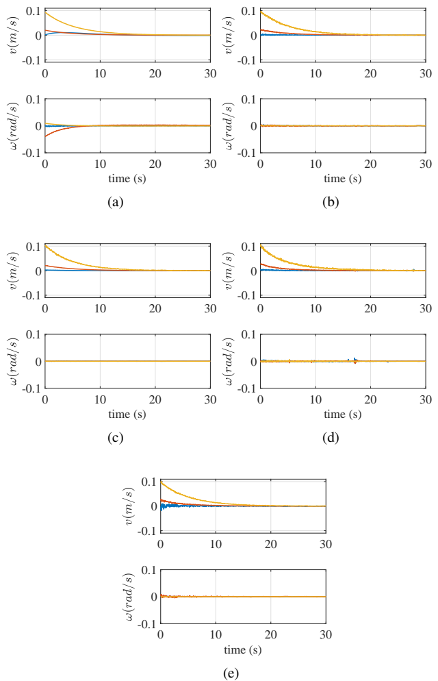
Figure 5. Experimental comparisons of the control inputs for: (a) method 1, (b) method 2, (c) method 3, (d) method 4, (e) and proposed approach in the pure translation case.
