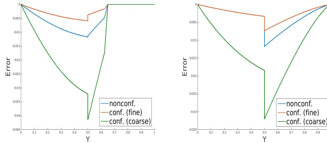
Figure 6.4: Example 1. Error in saturation along a line orthogonal to the interface, nonconforming and conforming (coarse and fine) time-steps. Left T = T_f/20 , right, T = T_f .
